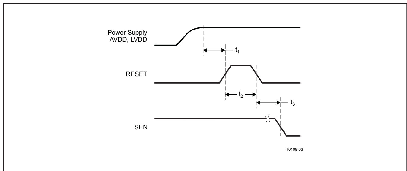
Figure 5. Reset Timing
