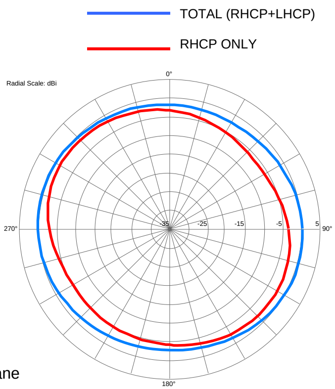
A10415-U1 Ref Board
