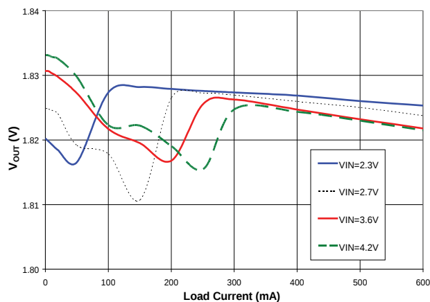
Figure 9. Load Regulation
