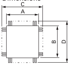
Outline IC Body Dimensions
