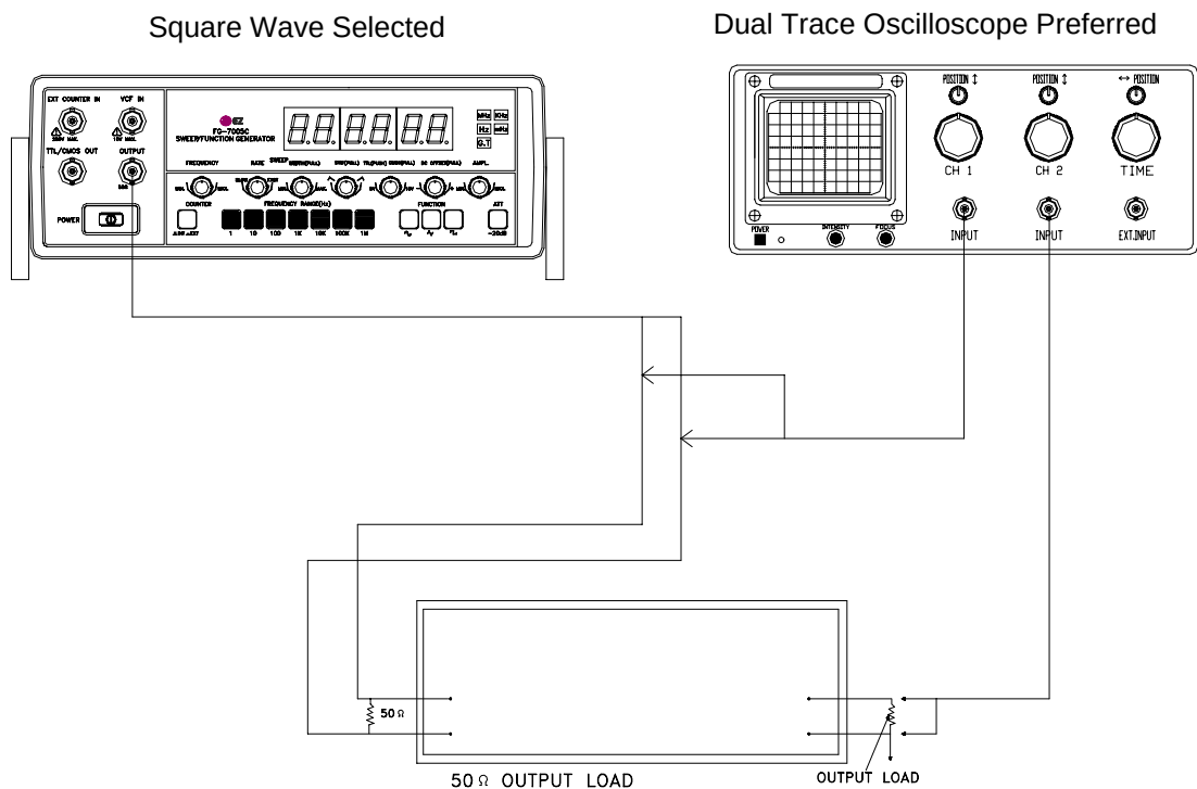
A. Test Waveforms
