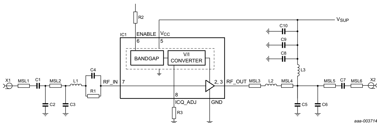
Fig 6. Application diagram of customer evaluation board for ISM-434 and ISM-915 application
