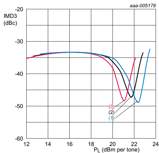
V_{SUP} = 3.6\text{ V} ; I_{CC(tot)} = 70\text{ mA} ; \Delta f = 1\text{ MHz} ; matched for ISM-915. (1) T_{amb} = -40\text{ °C} (2) T_{amb} = +25\text{ °C} (3) T_{amb} = +85\text{ °C}
