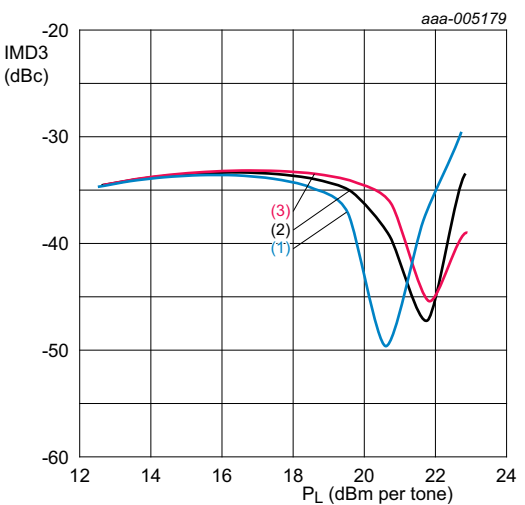
T_{amb} = 25\text{ °C} ; I_{CC(tot)} = 70\text{ mA} ; \Delta f = 1\text{ MHz} ; matched for ISM-915. (1) V_{SUP} = 3.3\text{ V} (2) V_{SUP} = 3.6\text{ V} (3) V_{SUP} = 3.9\text{ V}
