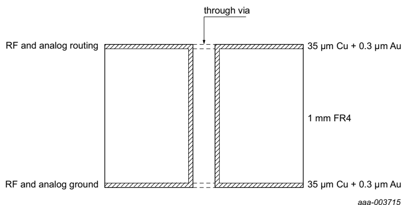
Fig 7. Printed-Circuit Board (PCB) stack build
