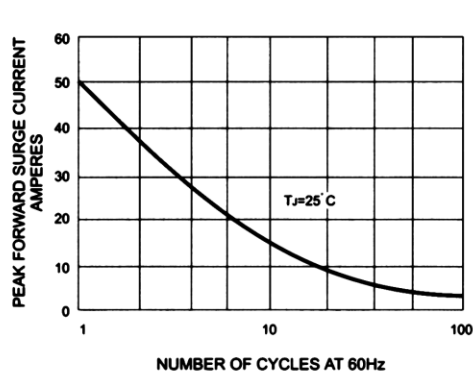
FIG. 1 - MAXIMUM FORWARD SURGE CURRENT
