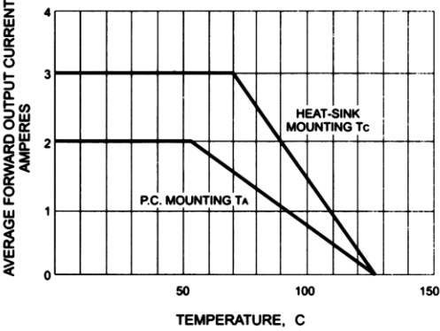
FIG. 2 - DERATING CURVE OUTPUT RECTIFIED CURRENT
