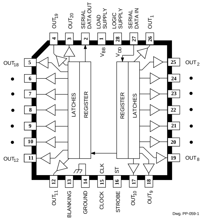
A6812xEP (PLCC)
