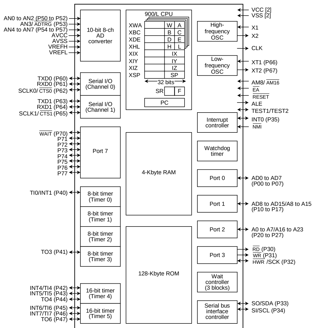
Figure 1.1 TMP93CW44 Block Diagram
