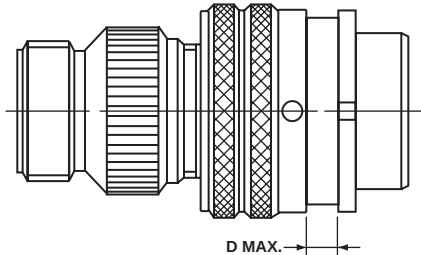
REAR MOUNTING DATA MAXIMUM PANEL THICKNESS
