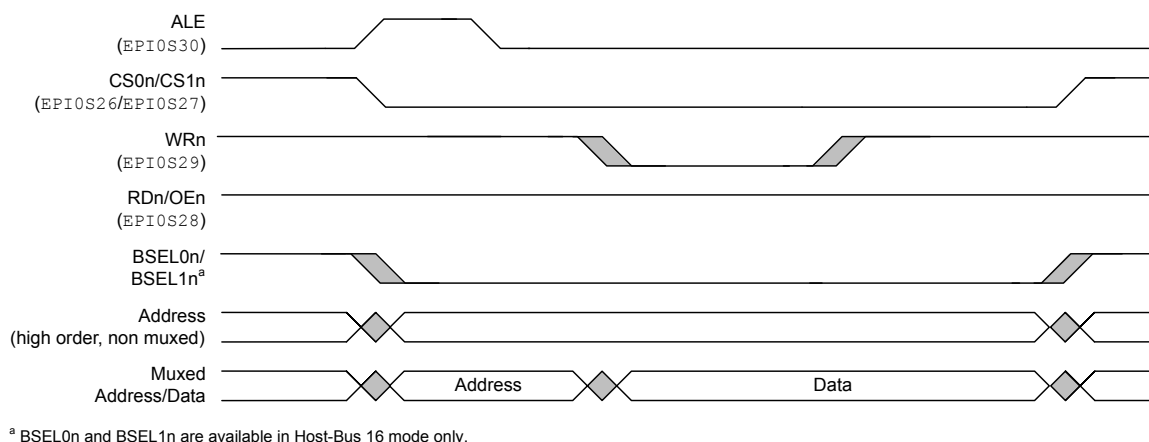
Figure 10-9. Host-Bus Write Cycle with Multiplexed Address and Data and ALE with Dual CSn
