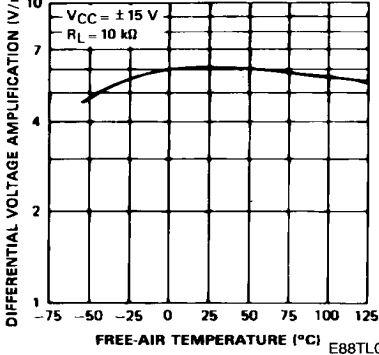
DIFFERENTIAL VOLTAGE AMPLIFICATION vs FREE-AIR TEMPERATURE
