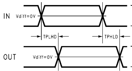
FIGURE 4. Propagation Delay Low-to-High and High-to-Low
