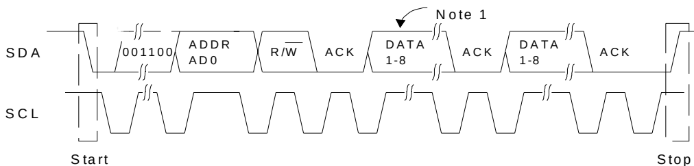
Figure 7. Control Port Timing, I²C Format
