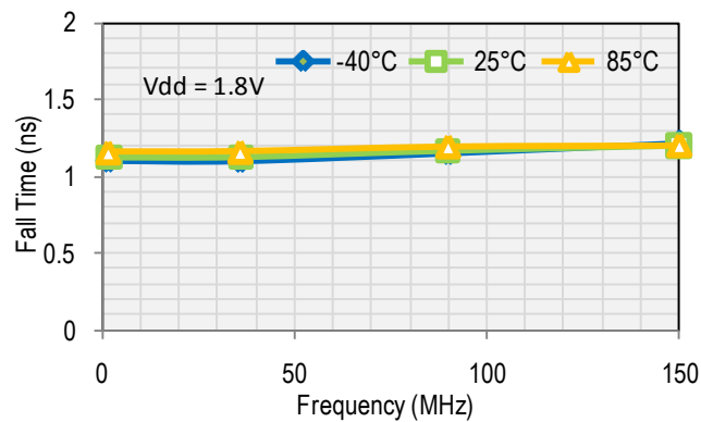
Fall Time
