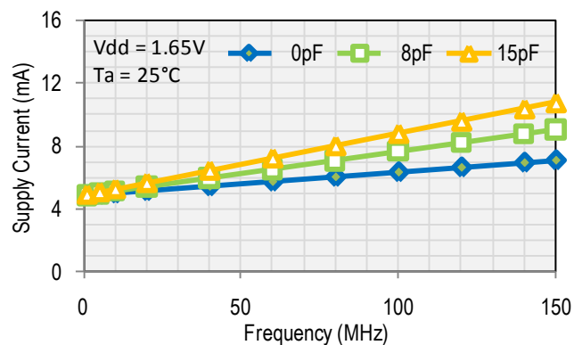
Supply Current
