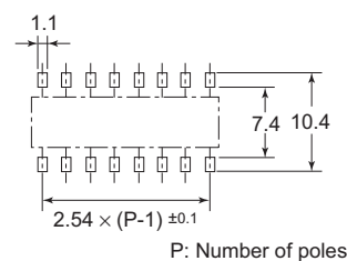
Dimensions of PCB Pad (Top View)
