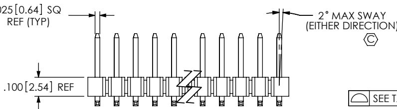
FIG 1 TSM-1XX-XX-XXX-DV SHOWN
