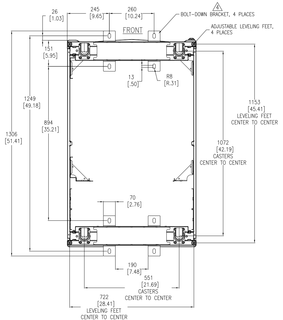
BOTTOM VIEW (WITH BOLT-DOWN BRACKETS FOR ANCHORING, SOLD SEPERATELY)
