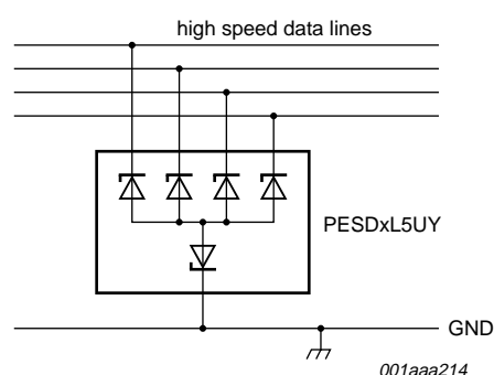
Fig.10 Typical application for bi-directional protection of four lines.
