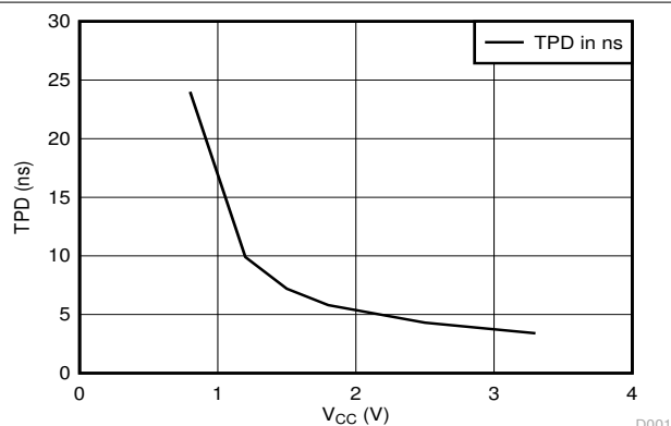
Figure 6-1. TPD vs V_{CC} , 15 pF Load
