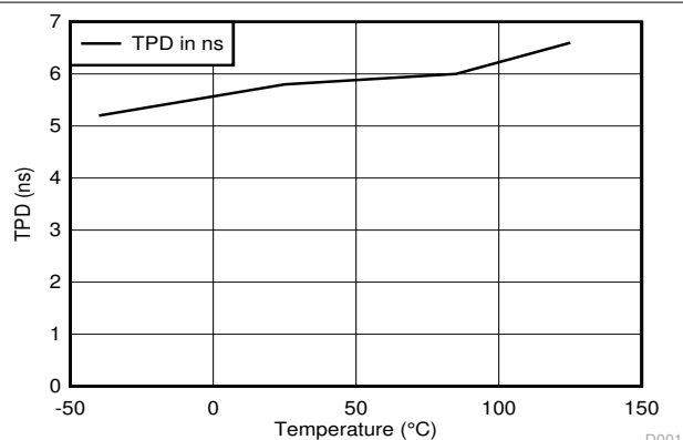
Figure 6-2. Temperature 1.8 V, 15 pF Load
