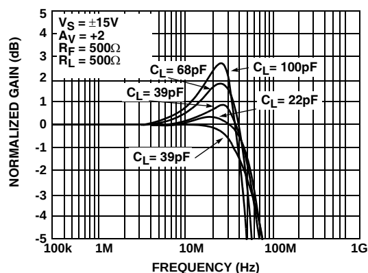
FIGURE 12. GAIN vs FREQUENCY FOR VARIOUS C_{LOAD} ( A_V = +2 )
