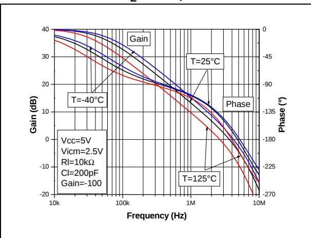
Figure 11. Voltage gain and phase with C_L = 200 \text{ pF}
