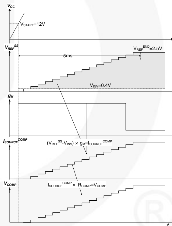
7. Soft-Start: When V_{CC} reaches V_{START} , the internal reference voltage is increased like a stair step for 5 ms. As a result, V_{COMP} is also raised gradually and MOSFET turn-on time increases smoothly. This reduces voltage and current stress on the power switch during startup.
