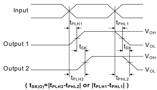
Figure 3. Output Skew
