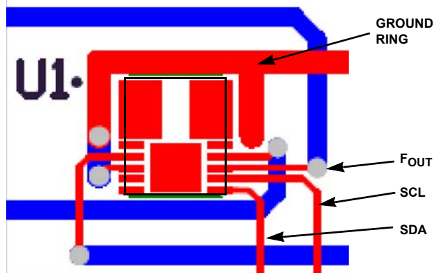
FIGURE 22. SUGGESTED LAYOUT FOR ISL12020M
