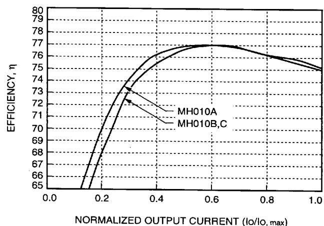
Figure 7. MH010A, B, C Typical Converter Efficiency as a Function of Output Current with V_I = 5\text{ V} and T_A = 25\text{ }^{\circ}\text{C}
