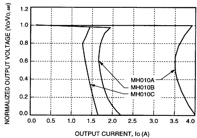
Figure 4. MH010A, B, C Typical Output Characteristics with V_i = 5\text{ V} , T_a = 25^\circ\text{C}
