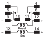
DC type
