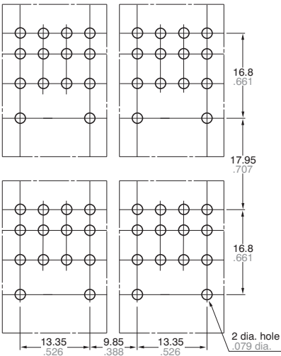
Side-by-side installation
