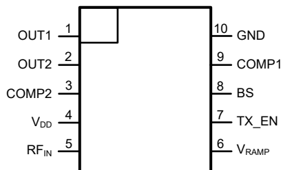
Figure 4-1. LMV242: NGY Package, WSON-10 (Top View)
