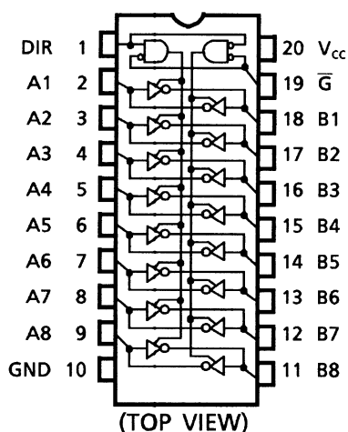
TC74HC640A
