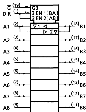
TC74HC245A
