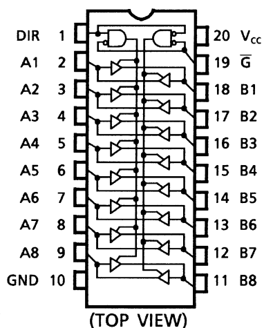
TC74HC245A
