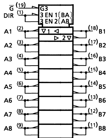
TC74HC640A
