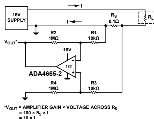
Figure 55. Low-Side Current Sensing Circuit
