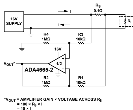
Figure 56. High-Side Current Sensing Circuit
