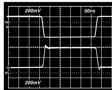
Figure 40. Receiver 400 mV Step Response, G = -1
