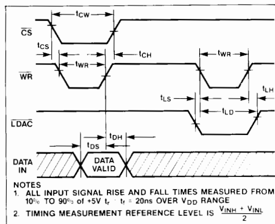
Figure 10. Write Cycle Timing Diagram
