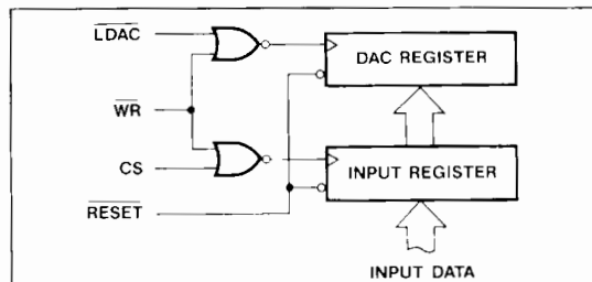
Figure 9. Input Control Logic
