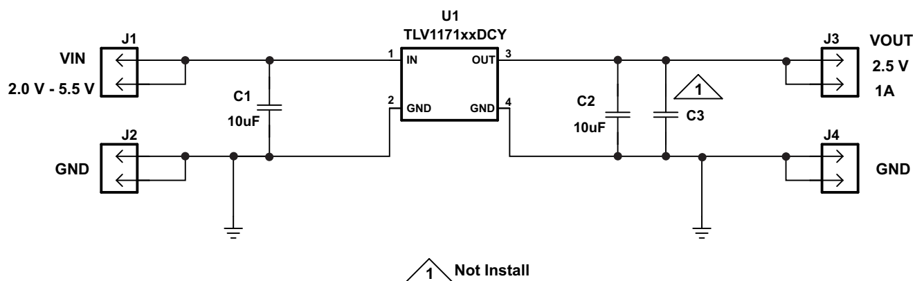
Figure 7. TLV117125EVM-097 Schematic
