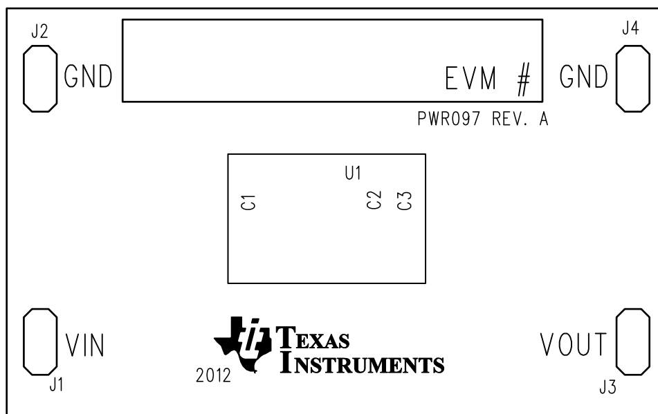
Figure 4. Assembly Layer
