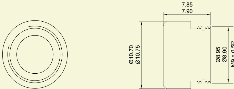
Interchangeable Line Lens (105° Fan Angle)
