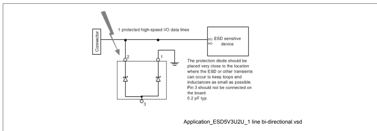
Figure 4-2 1 line, bi-directional TVS protection
