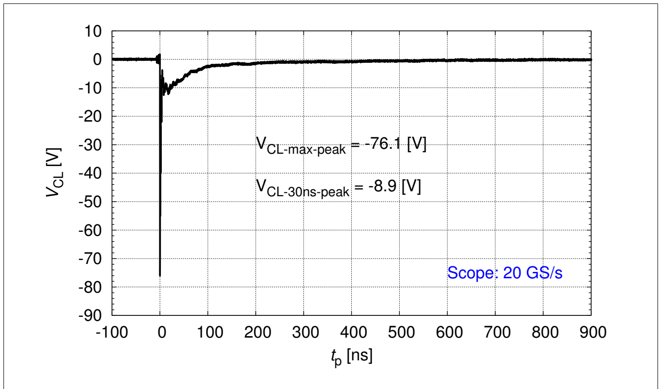
Figure 3-6 IEC61000-4-2: V_{CL} = f(t) , 8 kV negative pulse from pin 1 to pin 2 ( R = 330 \Omega , C = 150 pF)
