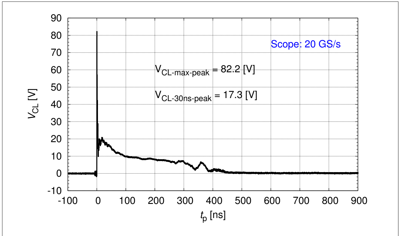
Figure 3-5 IEC61000-4-2: V_{CL} = f(t) , 8 kV positive pulse from pin 1 to pin 2 ( R = 330 \Omega , C = 150 pF)
