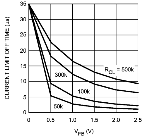
FIGURE 5. Current Limit Off-Time vs V_{FB} and R_{CL}
