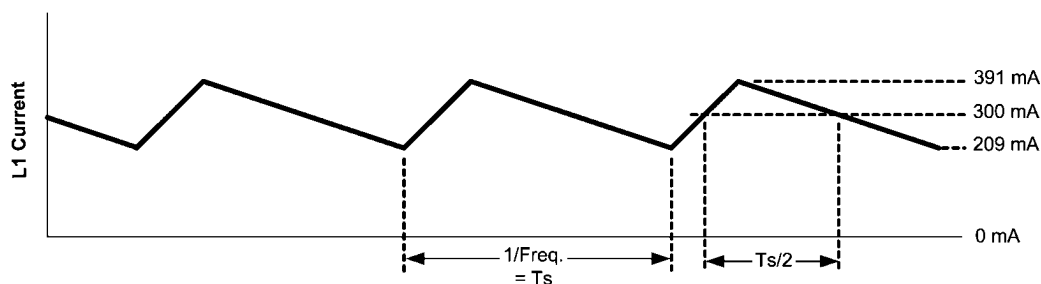
FIGURE 12. Inductor Current Waveform
