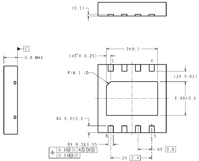
8-Lead LLP Package NS Package Number SDC08B
