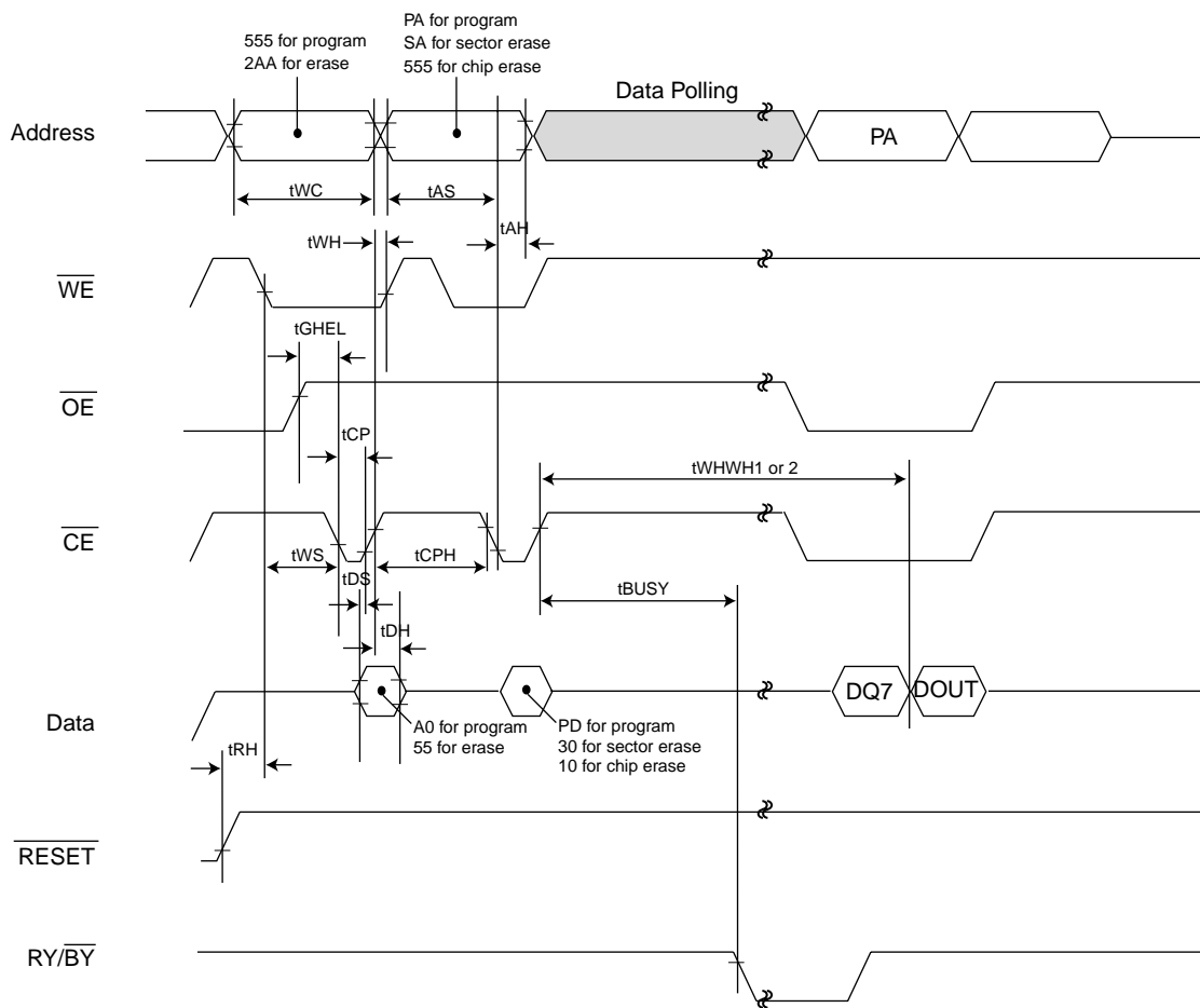
Figure 5. \overline{\text{CE}} CONTROLLED PROGRAM TIMING WAVEFORM
