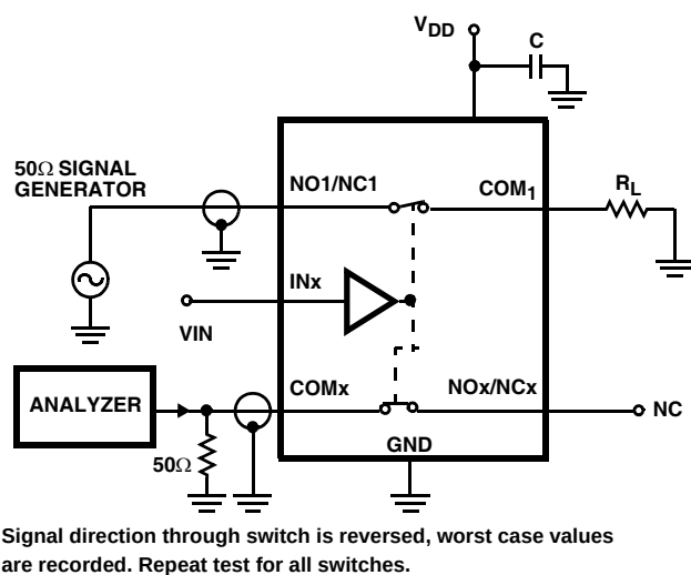
FIGURE 4. CROSSTALK TEST CIRCUIT
