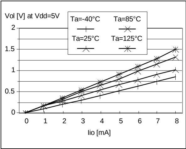
Figure 92. Typical V_{OL} at V_{DD}=5V ( \overline{\text{RESET}} )
