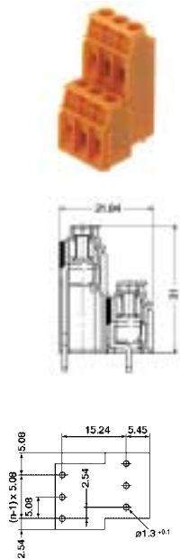
LP2N 5.08/90
