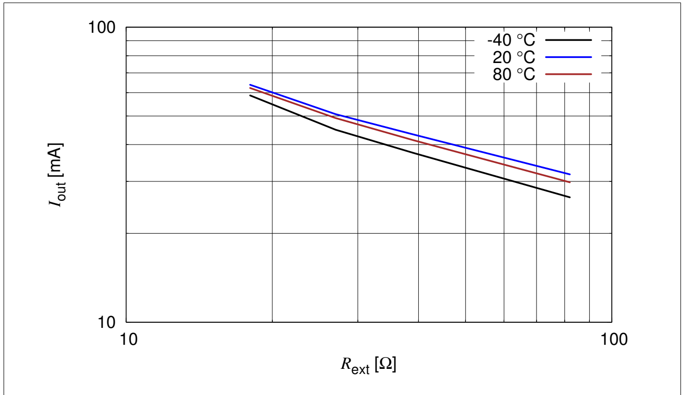
Figure 3-8 Output Current versus R_{ext} I_{out} = f(R_{ext}) , V_S = 10 V, V_S - V_{out} = 1.4 V, T_A = Parameter
