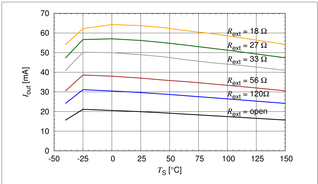
Figure 3-9 Output Current versus T_S I_{out} = f(T_S) , V_S = 10 V, V_S - V_{out} = 1.4 V, R_{ext} = Parameter
