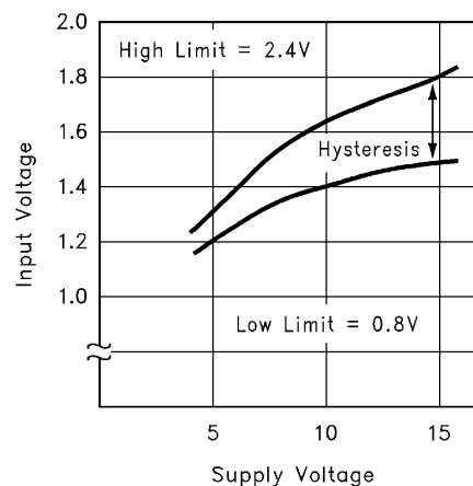
FIGURE 2. SWITCH THRESHOLD vs SUPPLY VOLTAGE
