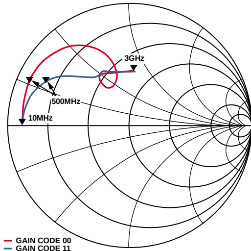
Figure 44. S_{22} (re: 50\ \Omega ) vs. V_{GAIN} over Gain Code for VGA2
