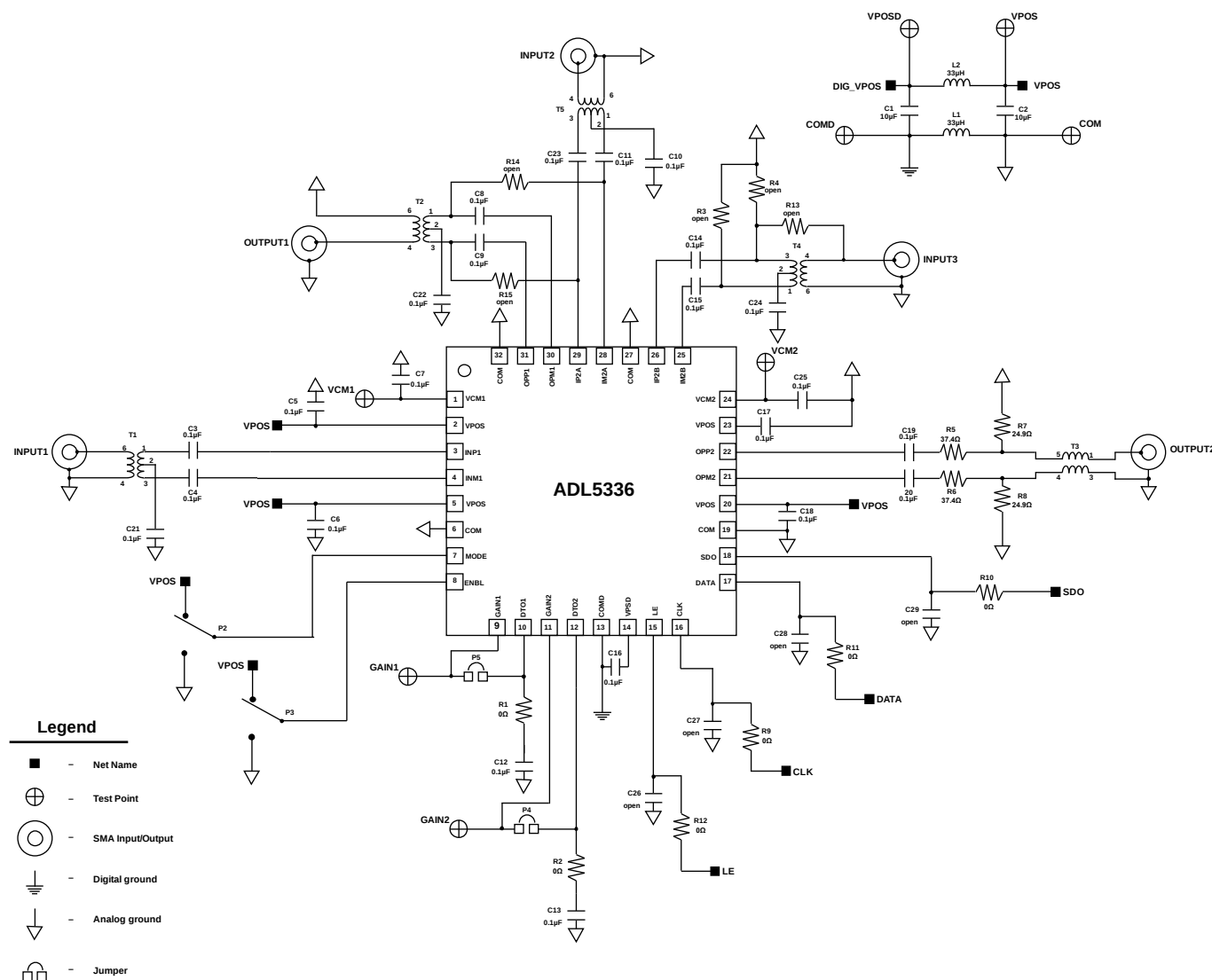
Figure 70. Evaluation Board Schematic
