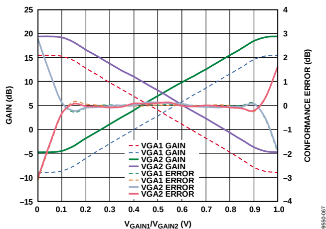
Figure 61. Gain and Conformance Error vs. V_{\text{GAIN1}}/V_{\text{GAIN2}} for Gain Code 11, and \text{MODE} = 0 \text{ V} and \text{MODE} = 5 \text{ V} for Both VGAs
