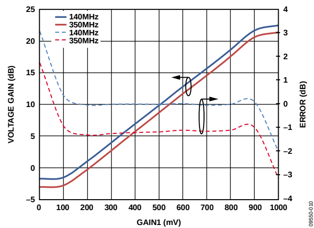
Figure 10. Gain vs. V_{\text{GAIN}} over Frequency at Gain Code 11 for VGA2
