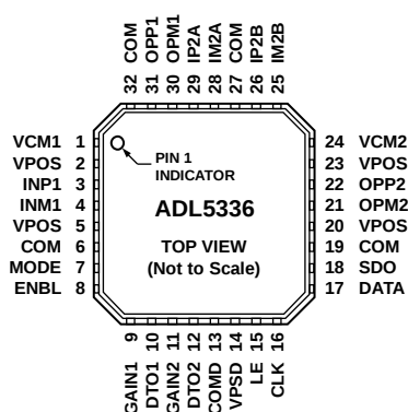
Figure 4. Pin Configuration
