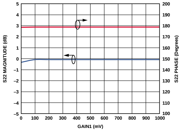
Figure 42. S_{22} (re: 200\ \Omega ) Magnitude and Phase vs. V_{GAIN} for VGA1
