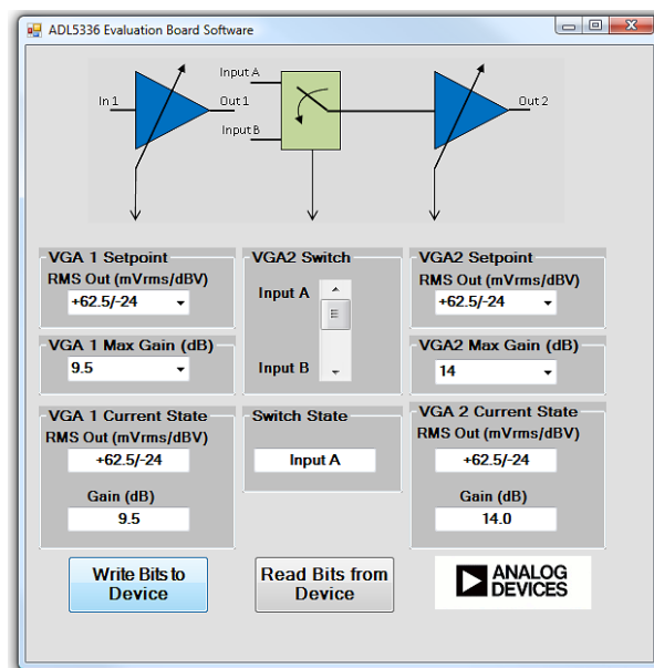
Figure 74. ADL5336 Software Screen Capture
