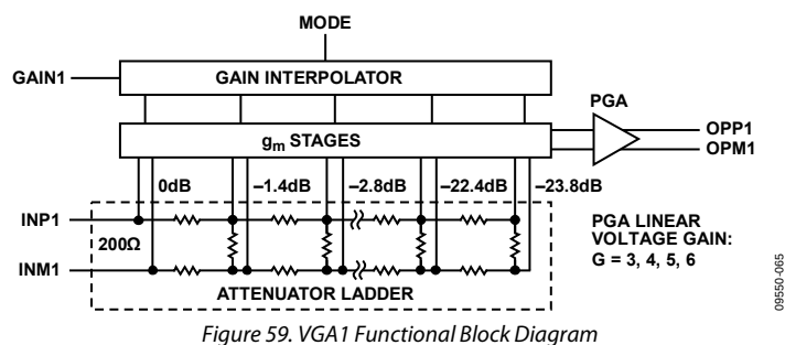
Figure 59. VGA1 Functional Block Diagram
