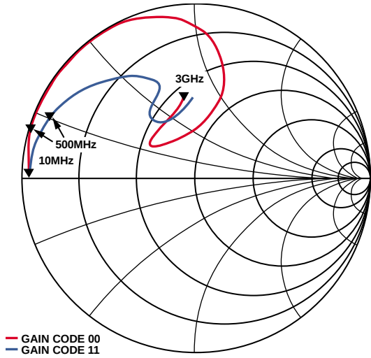
Figure 41. S_{22} (re: 50\ \Omega ) vs. V_{GAIN} over Gain Code for VGA1
