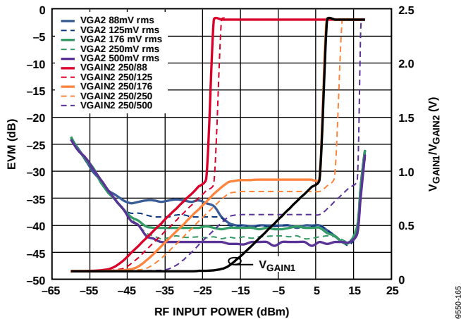
Figure 67. EVM vs. RF Input Power While VGA1 Setpoint Held Constant to 250 mV rms and VGA2 Setpoint Swept; VGA1/VGA2 Gain Code = 11
