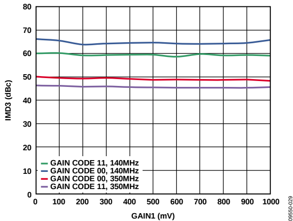
Figure 29. IMD3 vs. V_{\text{GAIN}} over Frequency and Gain Code, V_{\text{OUT}} = 1 \text{ V p-p} Composite, 2 MHz Spacing for VGA1
