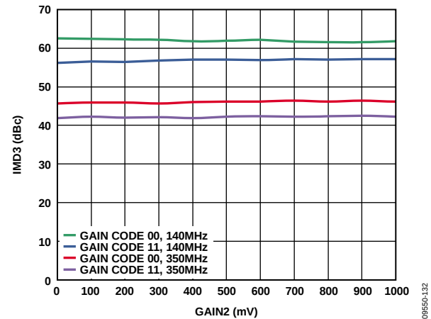
Figure 32. IMD3 vs. V_{\text{GAIN}} over Frequency and Gain Code, V_{\text{OUT}} = 1 \text{ V p-p} Composite, 2 MHz Spacing for VGA2
