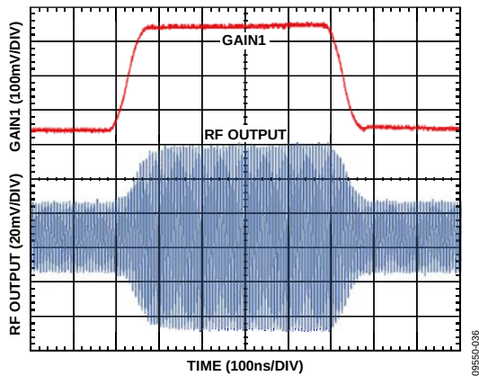
Figure 30. V_{\text{GAIN}} Step Response (VGA Mode) over Gain Step, V_{\text{IN}} = 100 \text{ mV p-p} for VGA1
