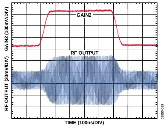
Figure 33. V_{\text{GAIN}} Step Response (VGA Mode) over Gain Step, V_{\text{IN}} = 100 \text{ mV p-p} for VGA2
