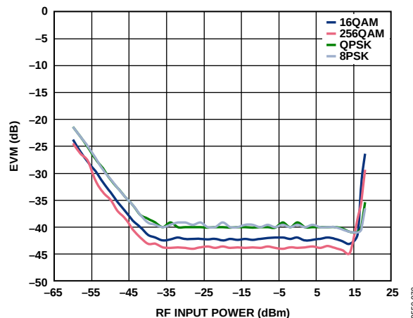
Figure 65. EVM vs. RF Input Power Over Several Modulation Types
