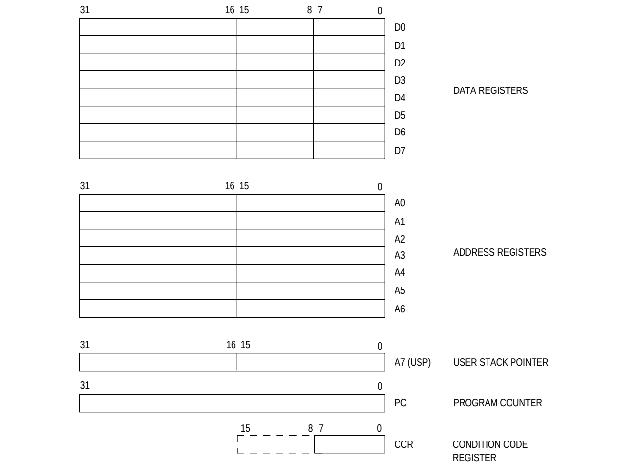
Figure 5-3. User Programming Model
