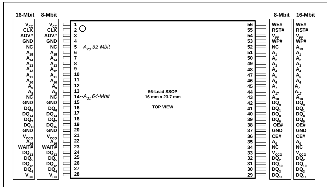
Figure 3. SSOP Pinout
