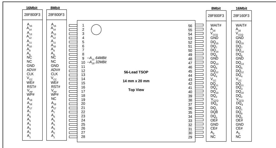
Figure 4. TSOP Pinout
