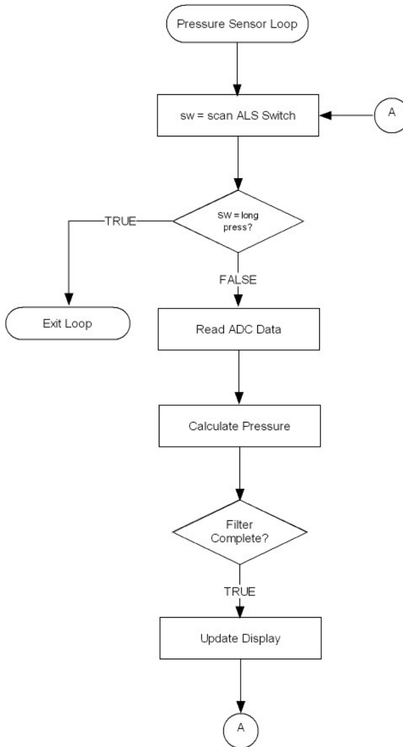
Figure 19. Flow of the Pressure Sensor Loop
