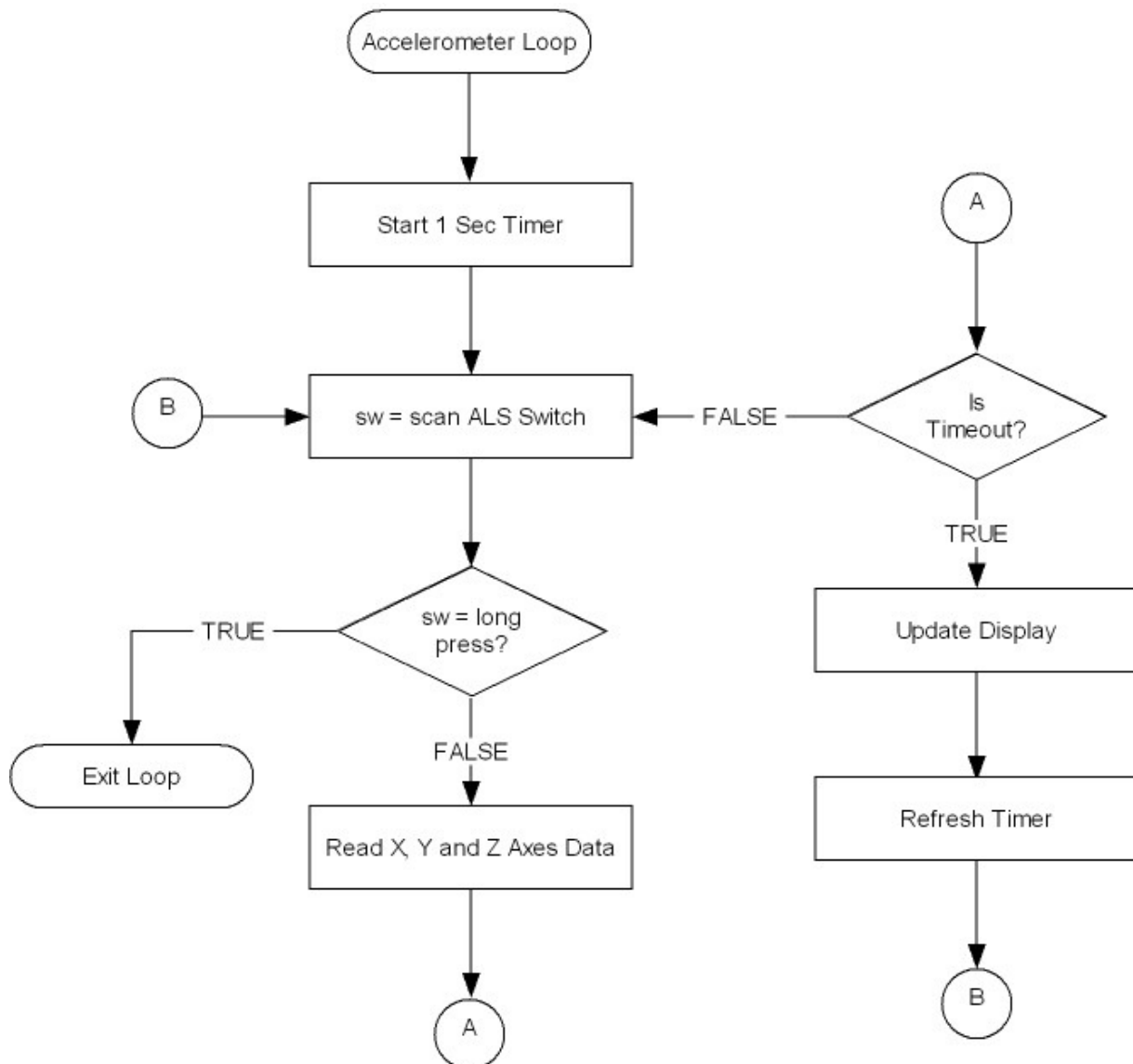
Figure 10. Flow of the Accelerometer Loop
