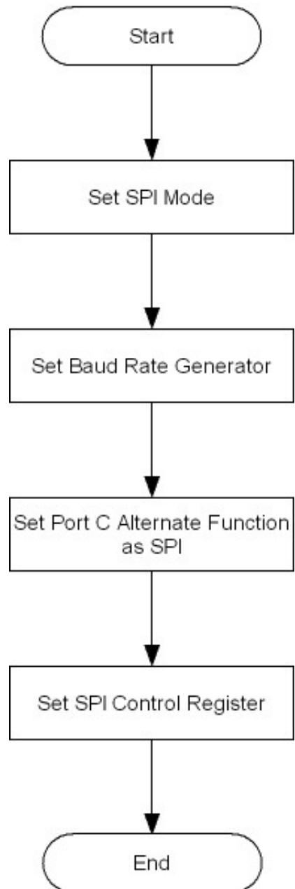
Figure 8. Flow of the SPI Initialization Function
