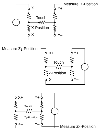
Figure 41. Pressure Measurement
