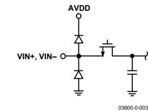
Figure 5. Equivalent Analog Input Circuit
