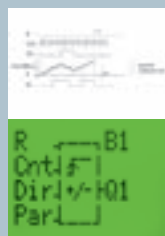
Up/down counter
