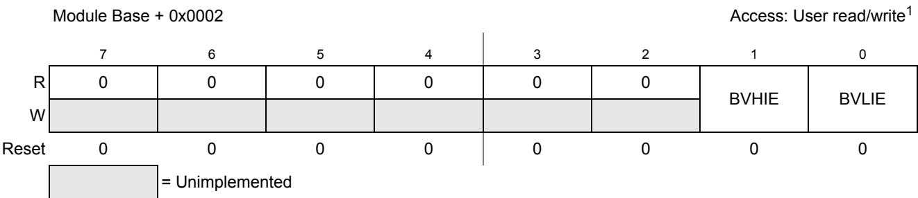
Figure 14-6. BATSV3 Interrupt Enable Register (BATIE)
