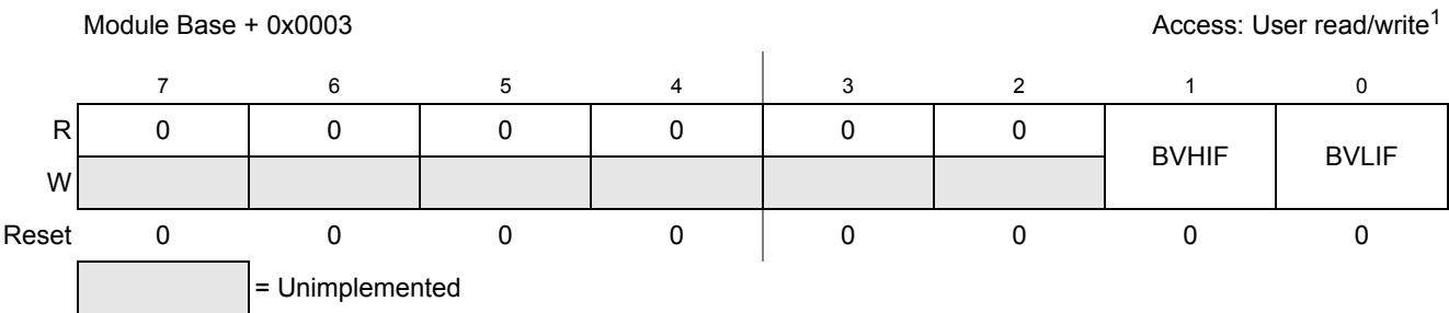
Figure 14-7. BATSV3 Interrupt Flag Register (BATIF)
