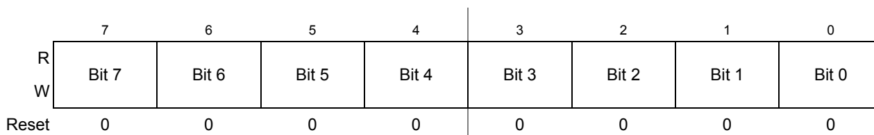
Figure 16-19. Timer Input Capture/Output Compare Register x Low (TCxL)
