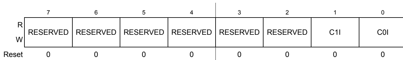
Figure 16-14. Timer Interrupt Enable Register (TIE)
