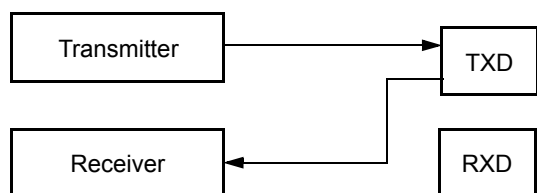
Figure 18-30. Single-Wire Operation (LOOPS = 1, RSRC = 1)
